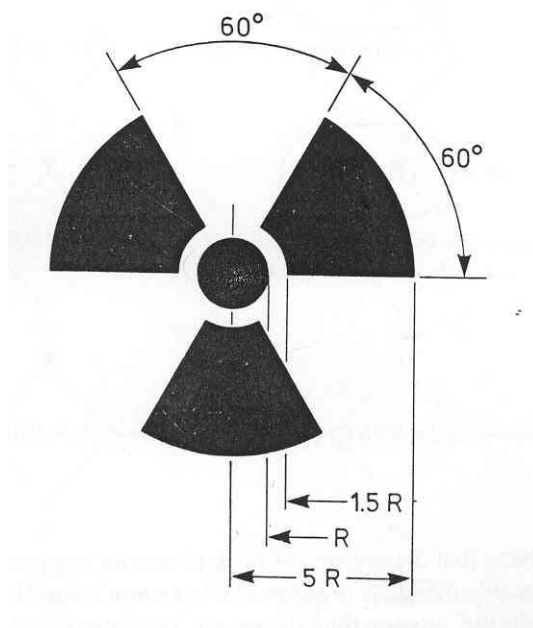
Fig 1 Basic symbol
